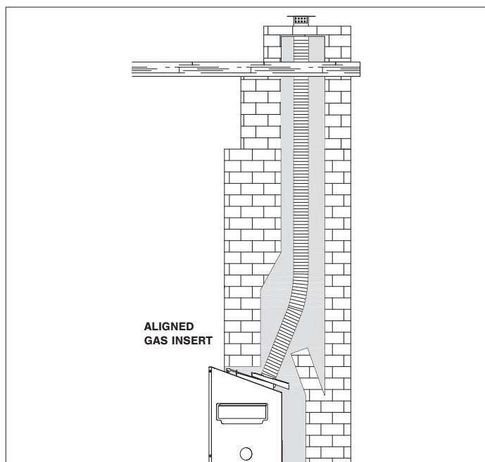
Figure 6.7, Aligned Gas Insert in Existing Fireplace
